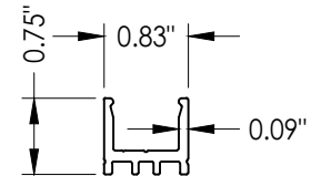
14 GLAZING STOP 9/16" Glazing
