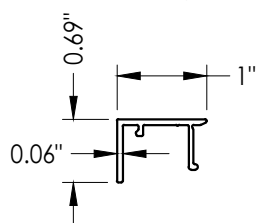
14 GLAZING STOP 9/16" Glazing
