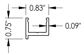
13 GLAZING STOP 1-5/16" Glazing
