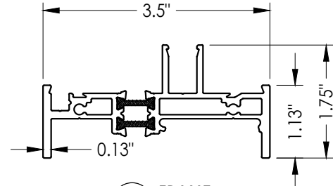
1 FRAME 9/16" Glazing
