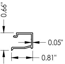
15 GLAZING STOP Interior Stained Glass
