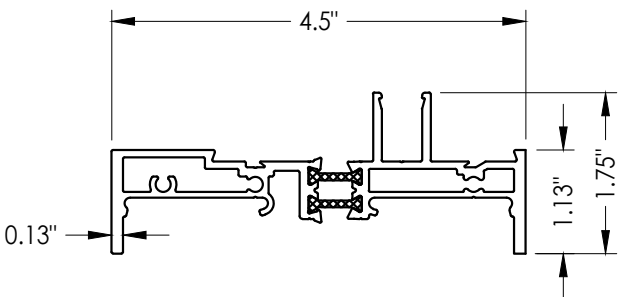
2 FRAME 1-5/16" Glazing
