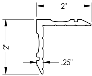
4 CORNER KEY
